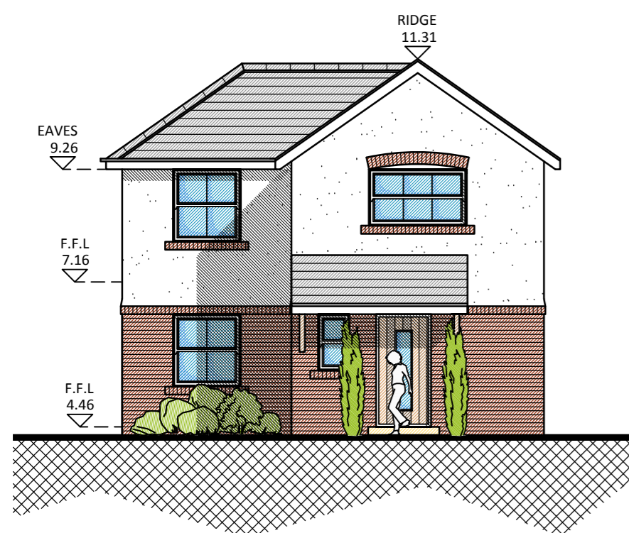
EAST ELEVATION SCALE 1:100
